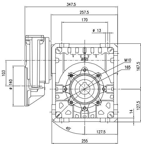
MOTOR COUPLING FLANGE, SIZE 90 B14 (24/140)
